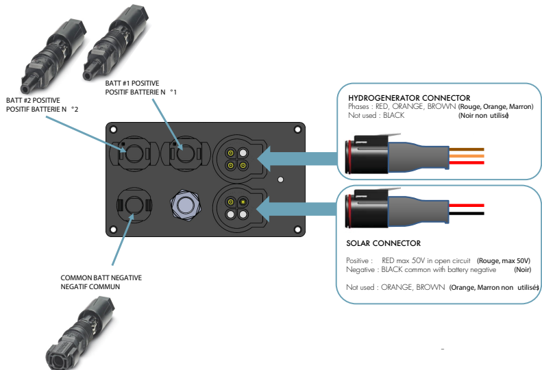
Converter connection
