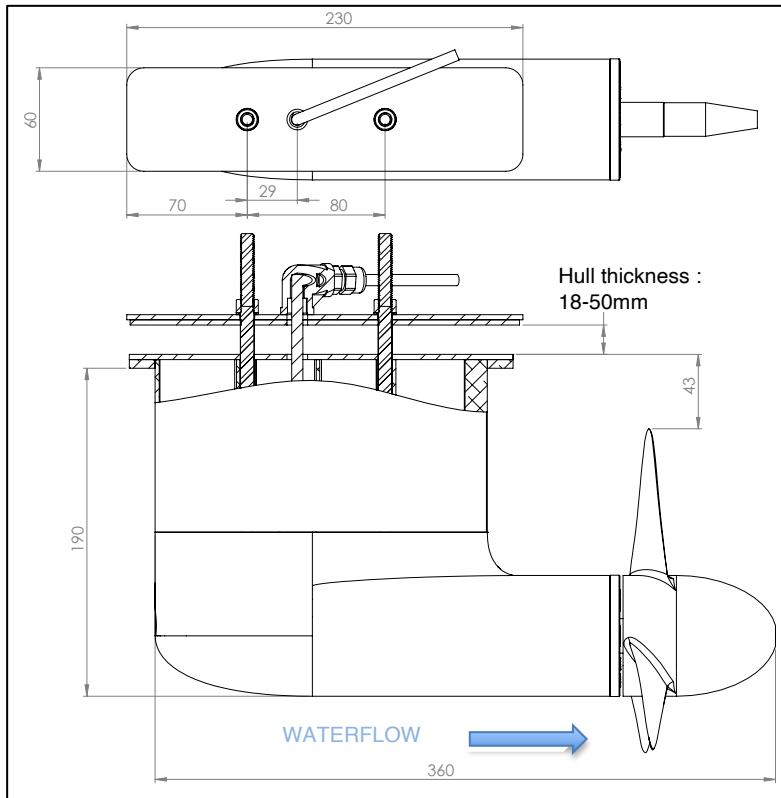
Dimensions of the POD 600 hydrogenerator in mm
