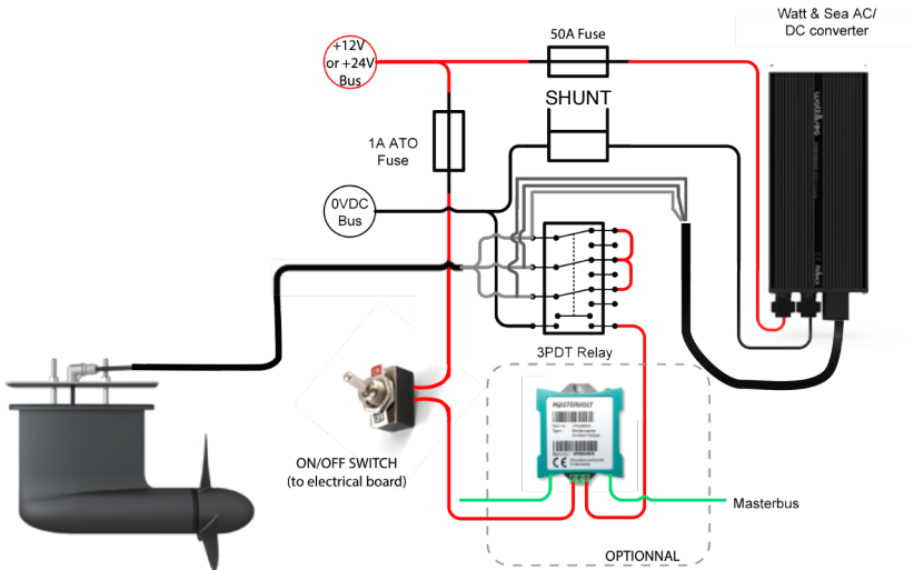
Wiring principle
